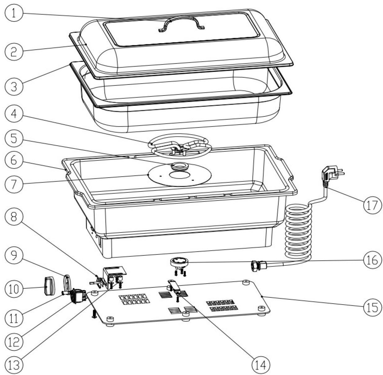
Exploded drawing for electric chafer
