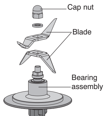
Blade assembly parts
