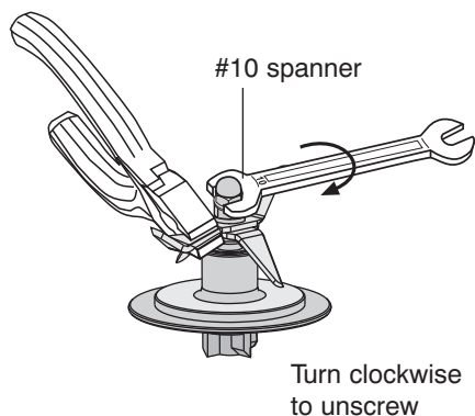
Disassembling blade
